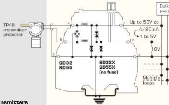
2-wire transmitters
